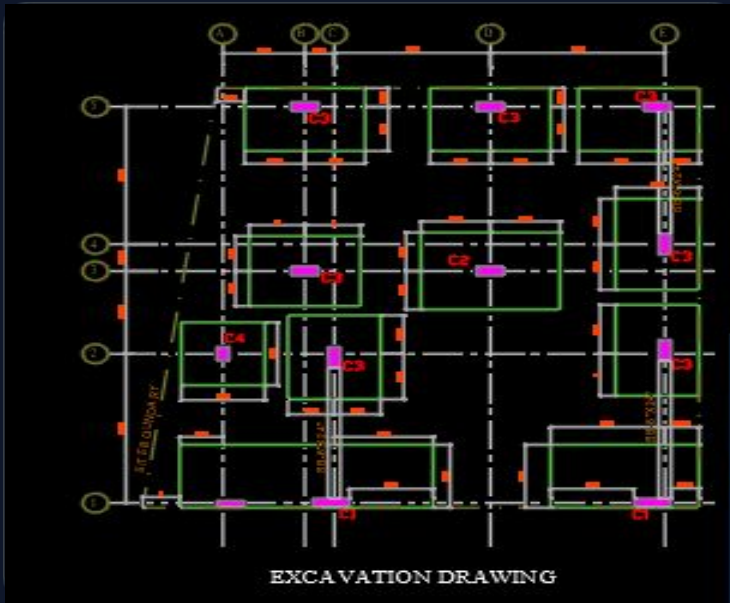
Footing Layouts
